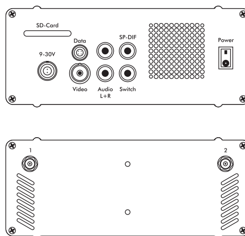
Anschlüsse // Connectors
